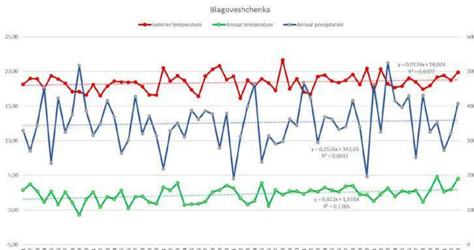
Figure 2 – Annual, summer temperature and annual precipitation at Meteo Station Blagoveshchenka
